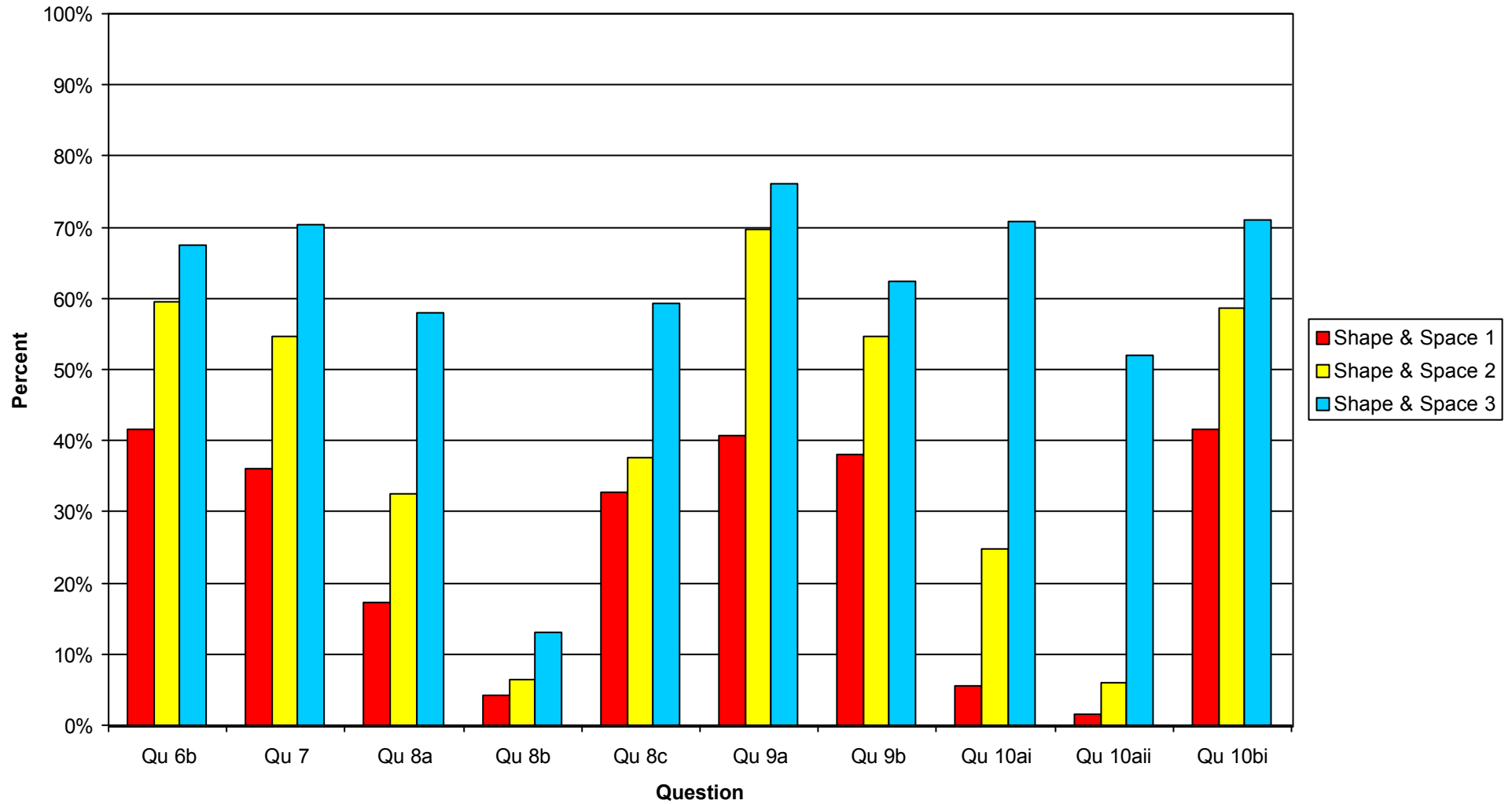
Germany Improvement in Shape & Space Question Responses
