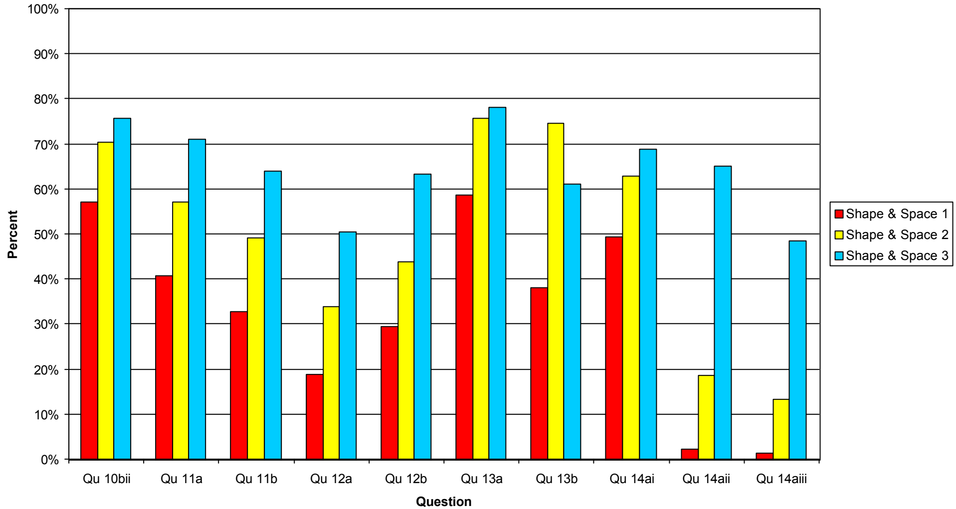
Germany Improvement in Shape & Space Question Responses
